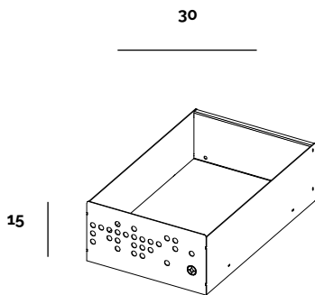
CASSETTO / DRAWER
