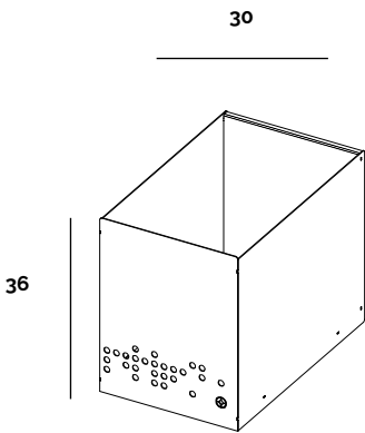
CASSETTO / DRAWER
